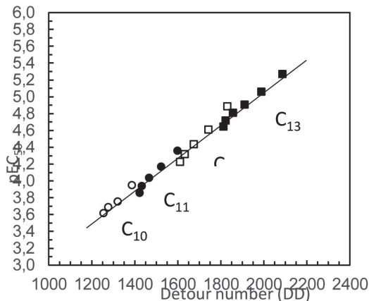
Figure 4. Correlation between detour number (DD) computed for various structural isomers of sodium salts of alkylbenzene sulfonates and experimental aquatic toxicity data (pEC 50 based on molar concentration) determined for goldfish
